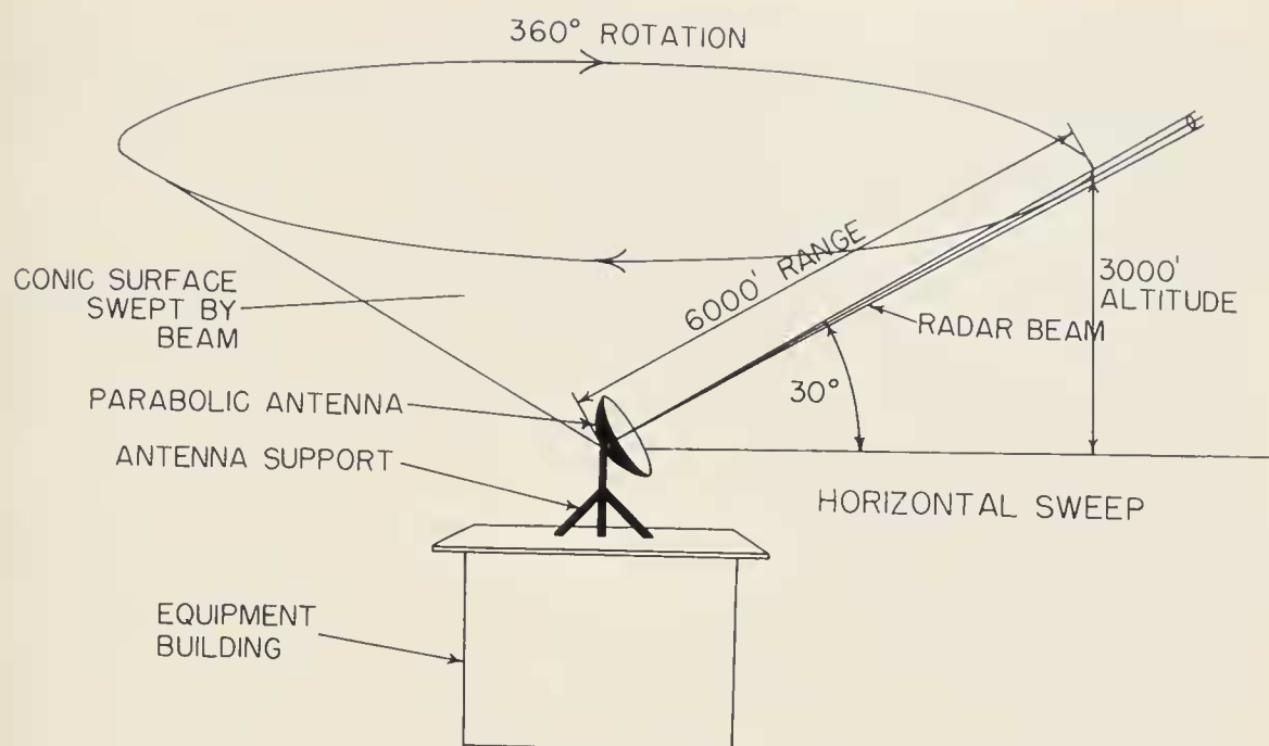
FIG. 2. Diagram showing 30^\circ (above horizontal) scan of radar antenna. Radar beam reaches upward one foot of altitude for every 2 feet of range.
